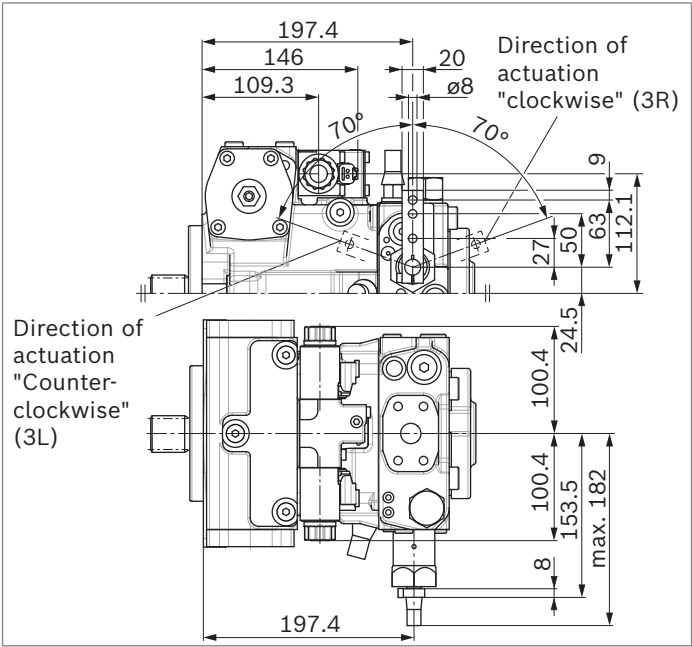
▼ DA..8 – Fixed setting and inch valve mounted
