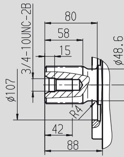
T Splined shaft 2 1/4 in 17T 8/16DP 3)
