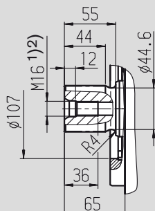
Z Splined shaft DIN 5480 W50x2x30x24x9g
