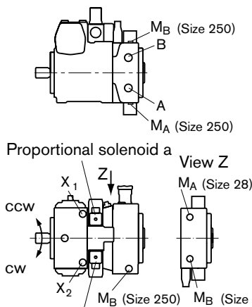
Proportional solenoid a
