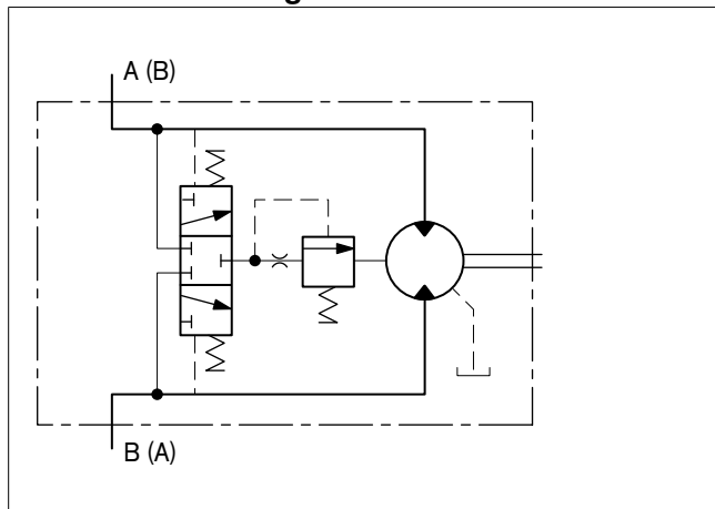
Motor with flushing valve
